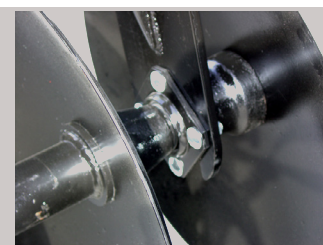
Heavy gang hanger with flange mounted triple sealed bearings
